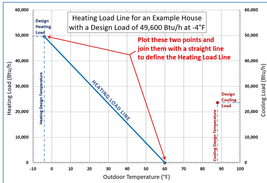
Figure 18: Example of a Plotting a Heating Load Line and Design Cooling Load for a House
